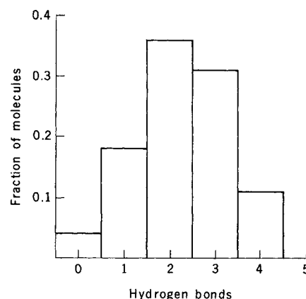
Fig. 5. Fractions of molecules in liquid water engaging in various numbers of hydrogen bonds. These results refer to the liquid at 10^\circ\text{C} and with a density of 1\text{ g/cm}^3 (17).
