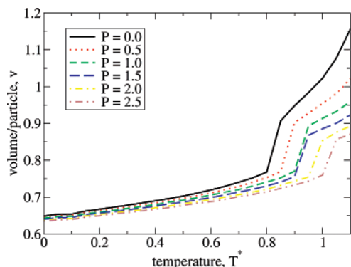
Figure 9. Specific volume as a function of temperature for a number of different pressure values for the three-dimensional Lennard-Jones system. These results are obtained from NPT Monte Carlo simulations with N = 864 particles and periodic boundary conditions. In its crystalline (fcc) state, this system expands when temperature is increased for all pressures and temperatures. Note that the “kinks” in the curves indicate melting of the crystal.
