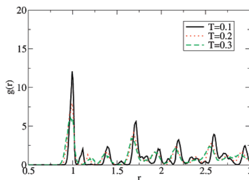
Figure 13. Radial distribution function for the SIC system in three dimensions at p = 1.0 for three temperatures, T^* = 0.1, 0.2, and 0.3 . As a result of the increasing curvature of the SIC potential, given in eq 6, near its minimum, the first peak is increasingly skewed to smaller r as the temperature is increased. The second peak is not present in the perfect fcc lattice and represents a shearing of the system.
