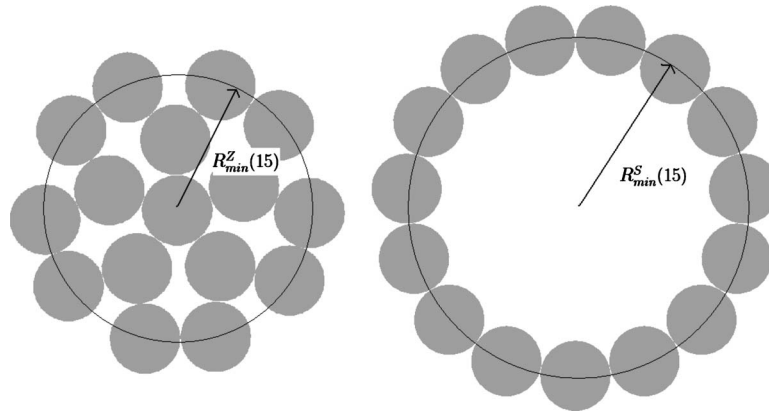
FIG. 1. Left: a conjectured optimal DLP configuration for N=15 , d=2 , and R_{\min}^Z(15)=1.873\,123\dots . Right: a spherical code optimal configuration for N=15 , d=2 , and R_{\min}^S(15)=1/(2\sin(\pi/15))=2.404\,867\dots
