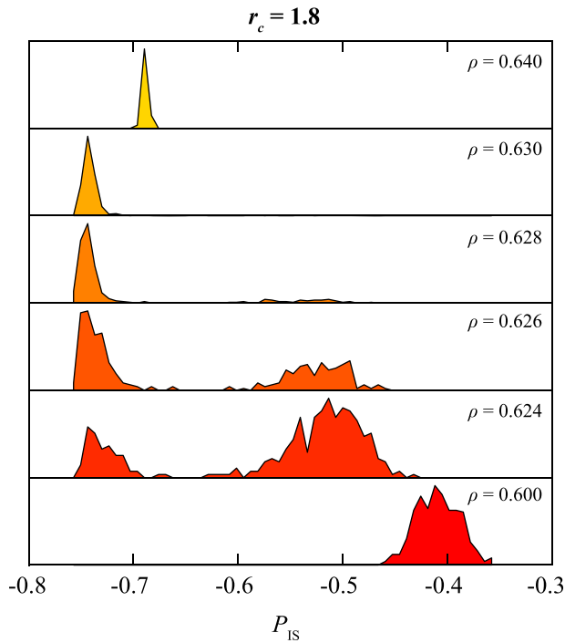
FIG. 3. Development of the inherent structure pressure distribution crossing the tensile instability at \rho_S for r_c = 1.8 ; N = 100\,000 . Below \rho_S , the distribution becomes bimodal, as the liquid samples both homogeneous and fractured inherent structures. At low enough density, all the inherent structures are fractured, and the pressure distribution is unimodal.
