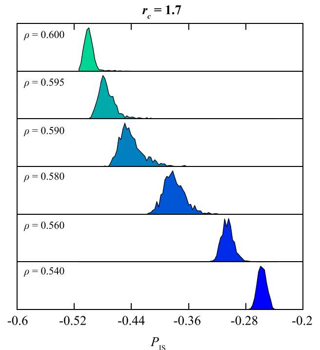
FIG. 6. Development of the inherent structure pressure distribution crossing the tensile instability at \rho_S for r_c = 1.7 ; N = 100\,000 . Below \rho_S , the distribution remains unimodal, and the entire distribution shifts to lower tension.
