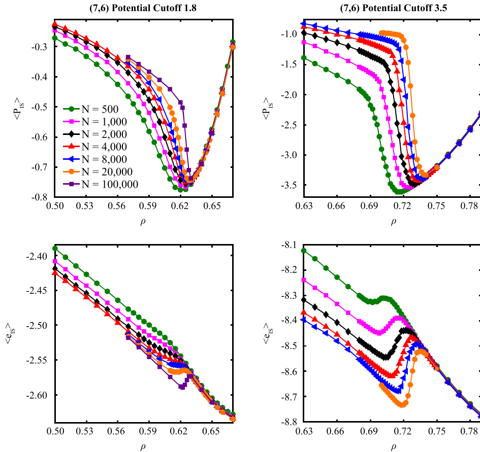
FIG. 2. Development of the landscape equation of state and the average potential energy per particle with system size for r_c = 1.8 and 3.5 . This range of cohesive strengths ( r_c \geq 1.8 ) exhibits strong finite-size effects, indicating the presence of a cavitation transition in the energy landscape.
