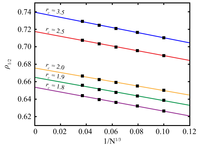
FIG. 4. Finite-size scaling of the cavitation transition for cutoffs within the strong cohesion regime.
