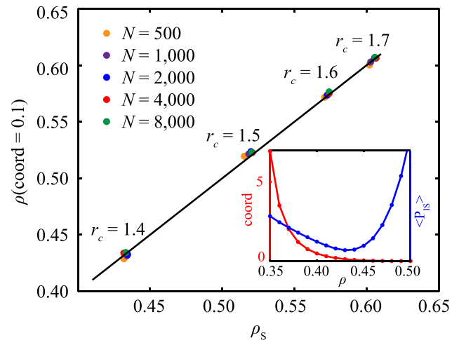
FIG. 11. The density where the average coordination number departs from zero (defined as 0.1 ) versus \rho_S , the density of tensile instability in the energy landscape, for cutoffs in the weakly cohesive regime. The coincidence of these two densities suggests that yielding in the energy landscape of weakly cohesive systems is due to the formation of a highly interconnected network of voids. The inset shows an example of the average coordination number plotted alongside the landscape equation of state for r_c = 1.4 .
