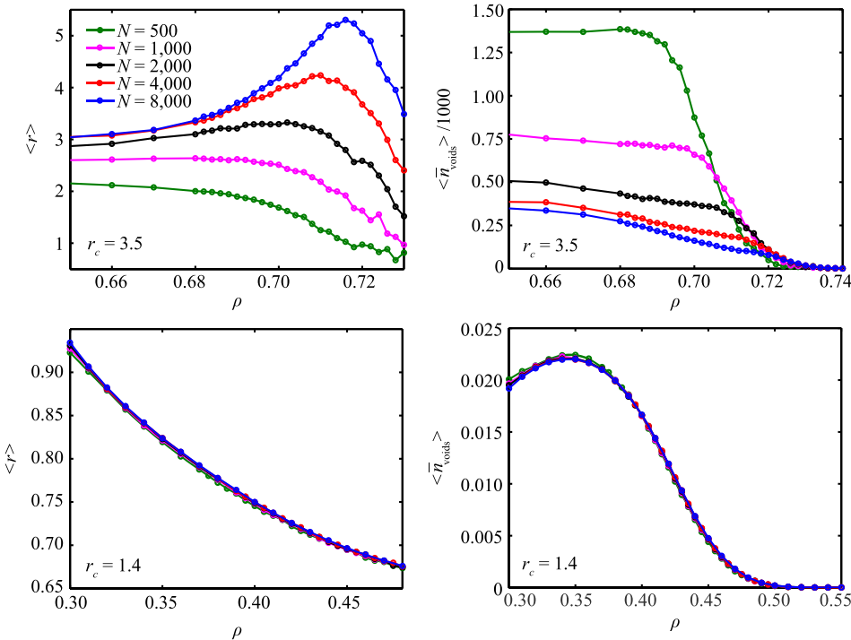
FIG. 7. Average void radius \langle r \rangle and number of voids per unit volume \langle \bar{n}_{voids} \rangle for r_c = 1.4 and 3.5.
