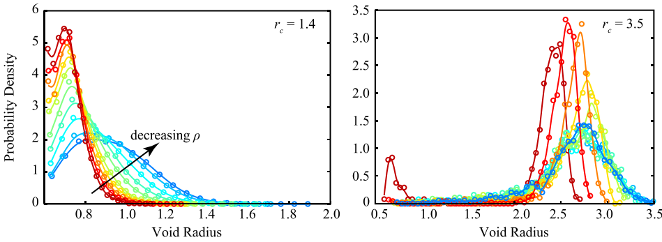
FIG. 9. Development of the void size distribution with density for r_c = 1.4 and 3.5 as the system is decompressed below \rho_S . The left panel displays densities between 0.30 and 0.43 , specifically: 0.30, 0.31, 0.33, 0.35, 0.37, 0.39, 0.40, 0.41, 0.42, and 0.43 . The right panel displays densities between 0.62 and 0.71 , incremented by 0.01 .
