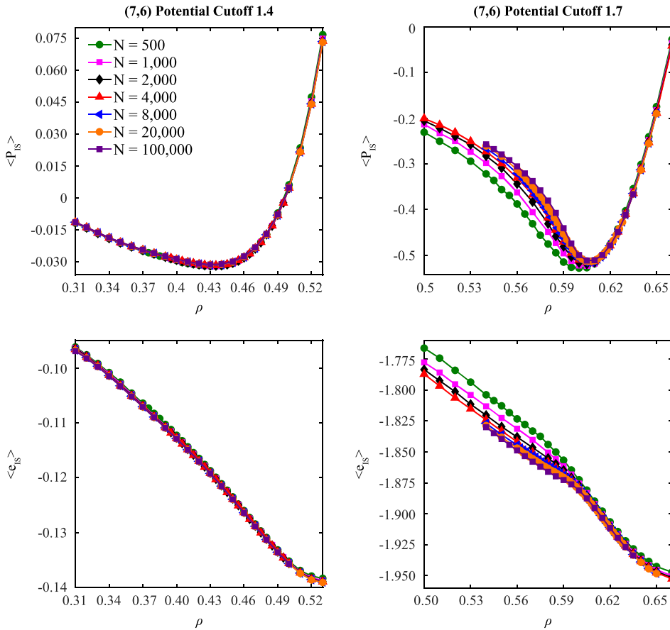
FIG. 5. Development of the landscape equation of state and the average potential energy per particle with system size for r_c = 1.4 and 1.7 . This range of cohesive strengths ( 1.4 \leq r_c \leq 1.7 ) exhibits minimal finite-size effects yet still displays a tensile instability in the energy landscape.
