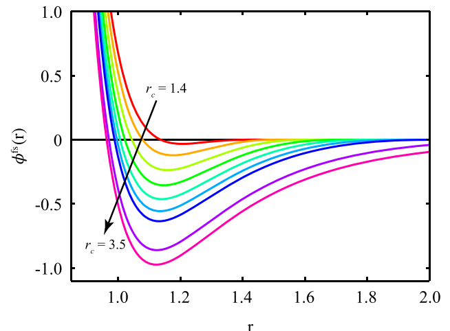
FIG. 1. Pair potential for each cutoff r_c considered in this work. Changing r_c changes the well depth and the extent of the attractive tail, allowing one to use r_c to tune the strength of particle cohesion.
