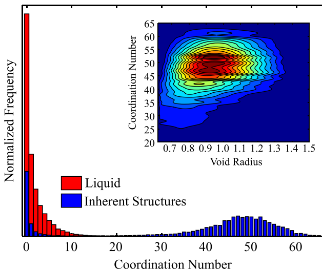
FIG. 10. Coordination number distribution of voids in the liquid and inherent structure for r_c = 1.4 at \rho = 0.31 , a density well below \rho_S . Energy minimization results in the formation of a highly interconnected network of small voids. Plotting the joint probability distribution of void size and coordination number of the inherent structures (inset) results in an “island” at high coordination number and small radius that is absent in the liquid.
